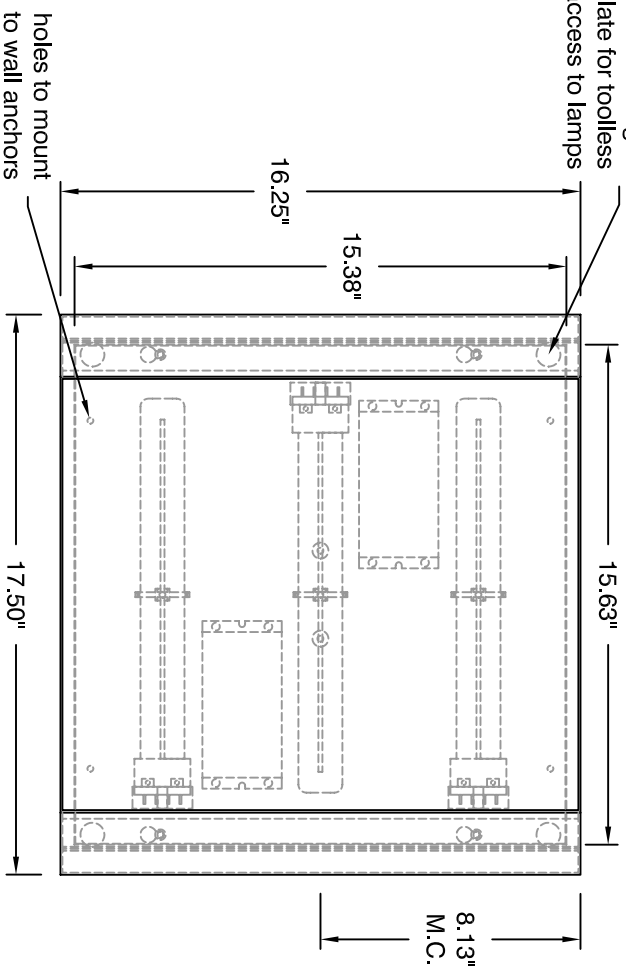
BOTTOM VIEW
