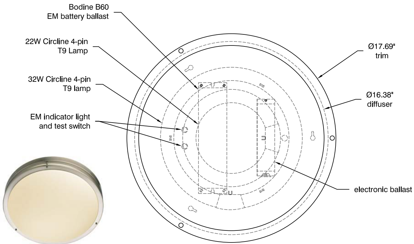
BOTTOM VIEW
